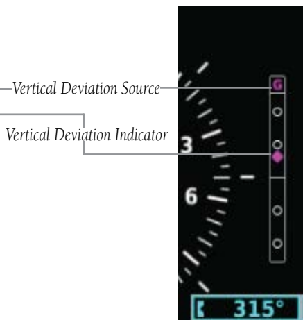
Figure 2-27 Vertical Deviation Indicator Position - HSI
