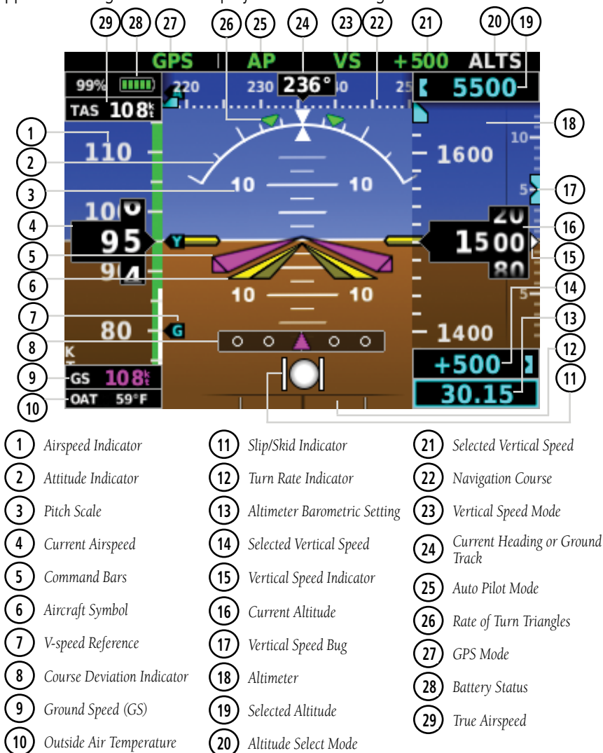
Figure 2-1 G5 PFD Flight Instruments
