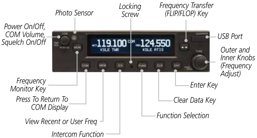
GTR 225 Front Panel Description
